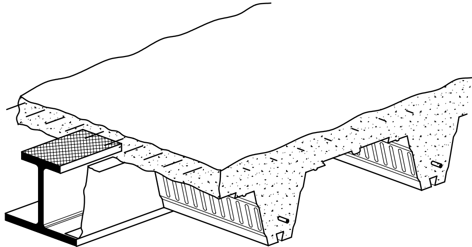
Figure 4.4 Slimdek construction
