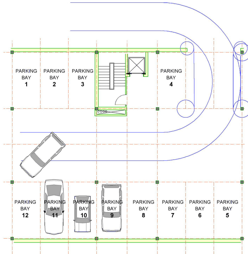
Figure 3.1 Typical arrangement for a basement car park in a residential multi-storey building
