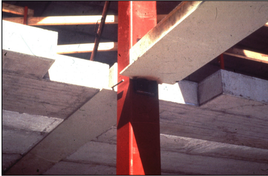
Figure 4.7 Slimflor beams supporting precast concrete slabs
