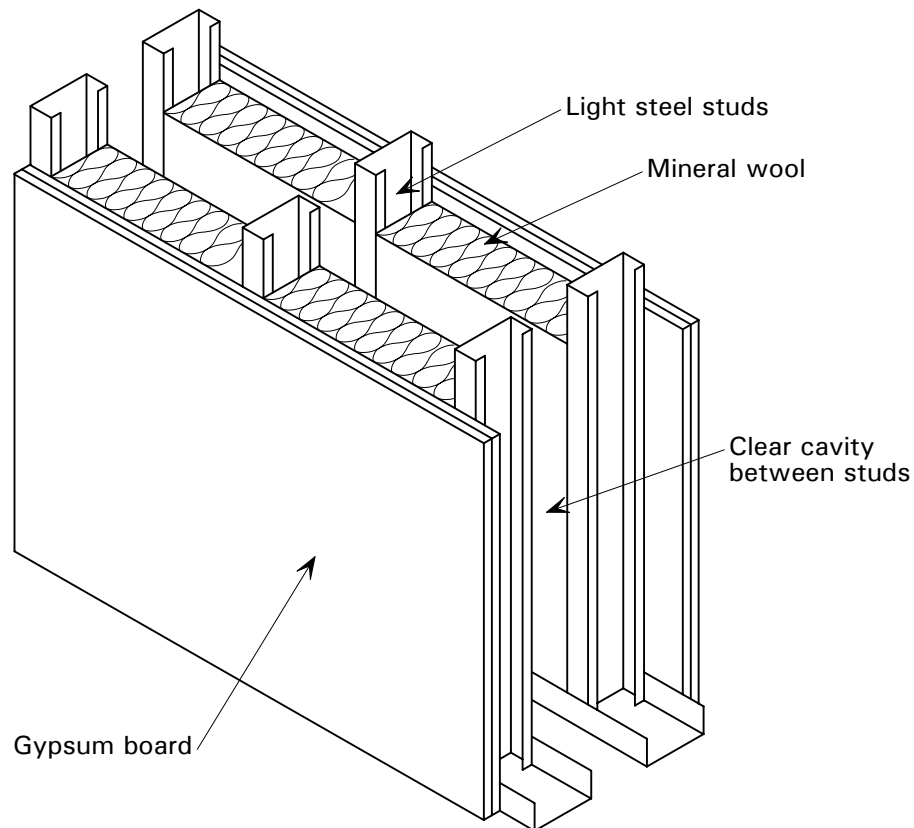
Figure 4.14 Typical light steel separating wall construction
