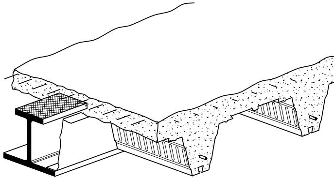
Figure 7.2 ASB with deep decking (composite beam)
