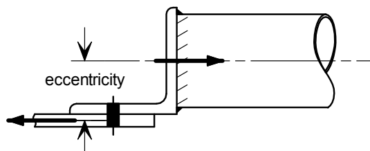
Figure 8.3 Eccentricity in connection to CHS
