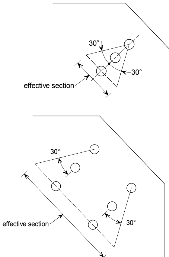
Figure 8.10 Effective section in tension
