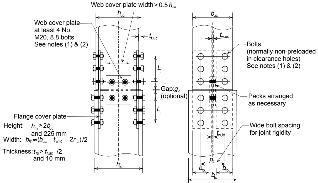
Axial compression developed in internal flange cover plates
