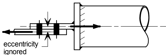
Figure 8.2 Lap joint between bracing and gusset
