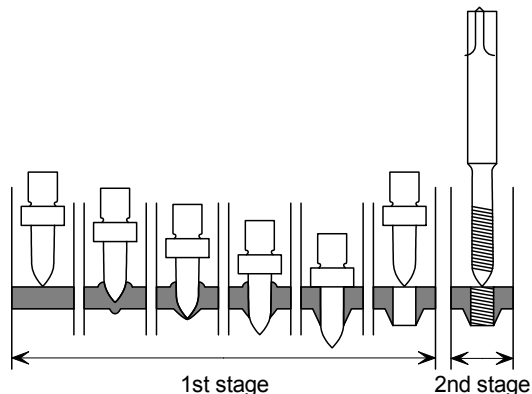
Figure D.2 Thermal drilling process
