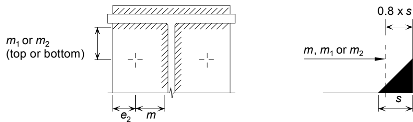
Setting out for Figure 7
