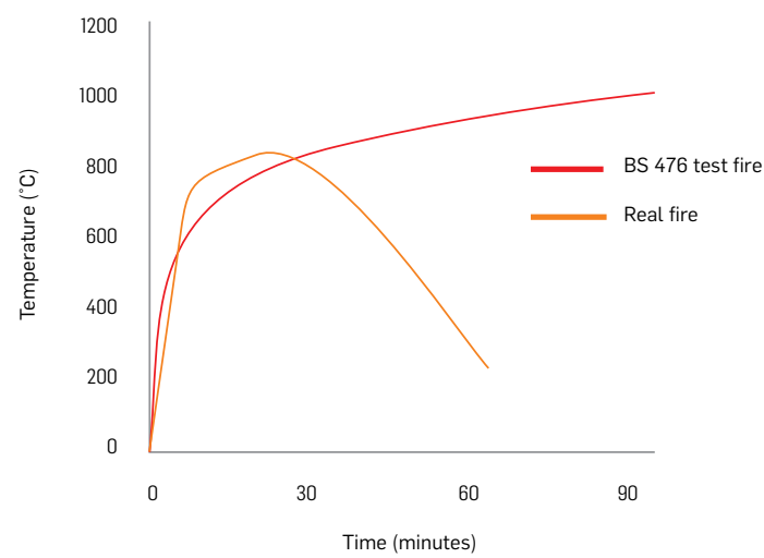
FIG 2. BEHAVIOUR OF FIRE IN TEST vs REAL FIRE
