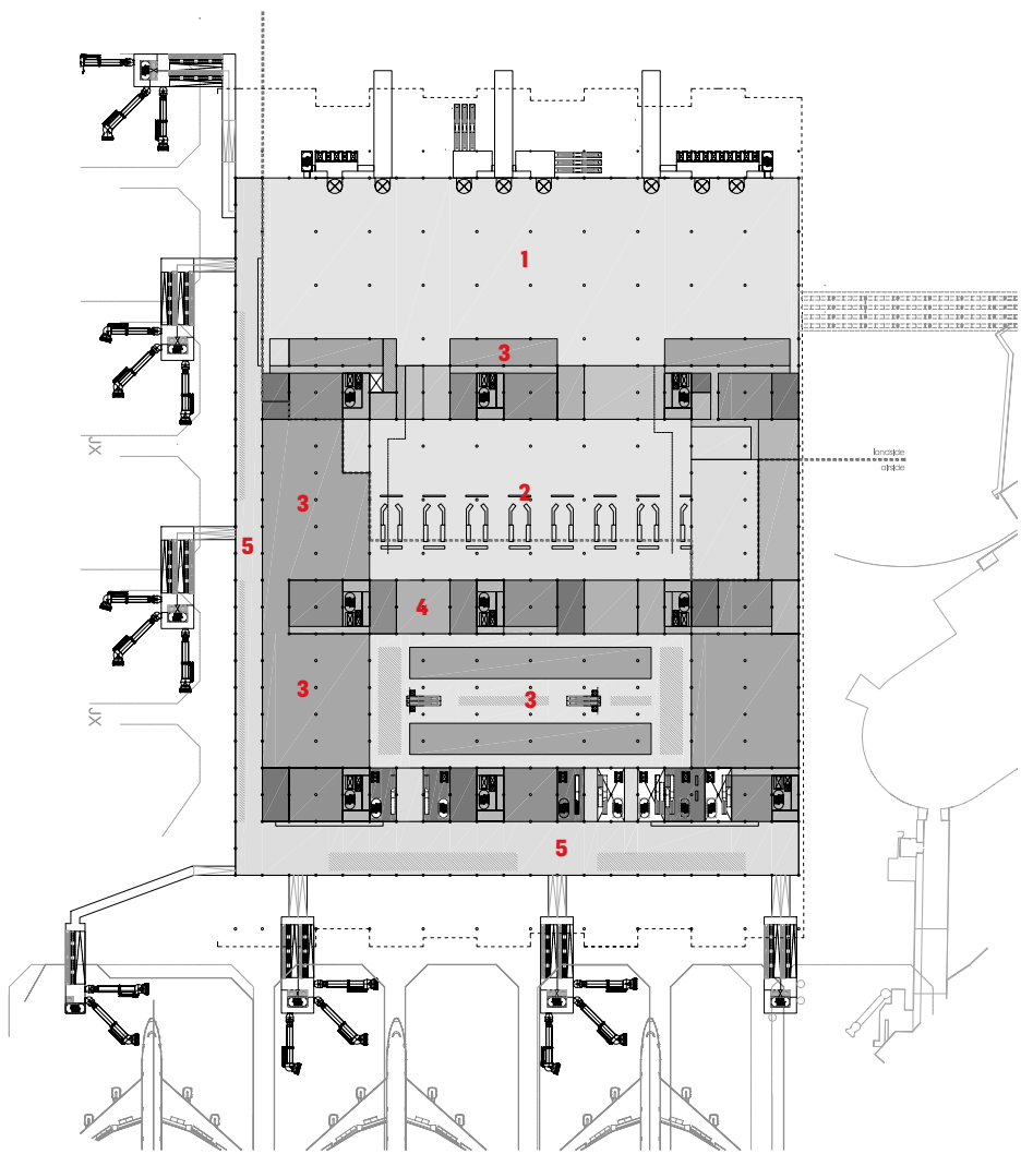
▲ PLAN: DEPARTURES LEVEL
