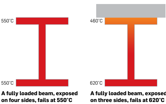
FIG 3. TEMPERATURE LIMITS FOR FULLY AND PARTIALLY EXPOSED STEEL BEAMS
