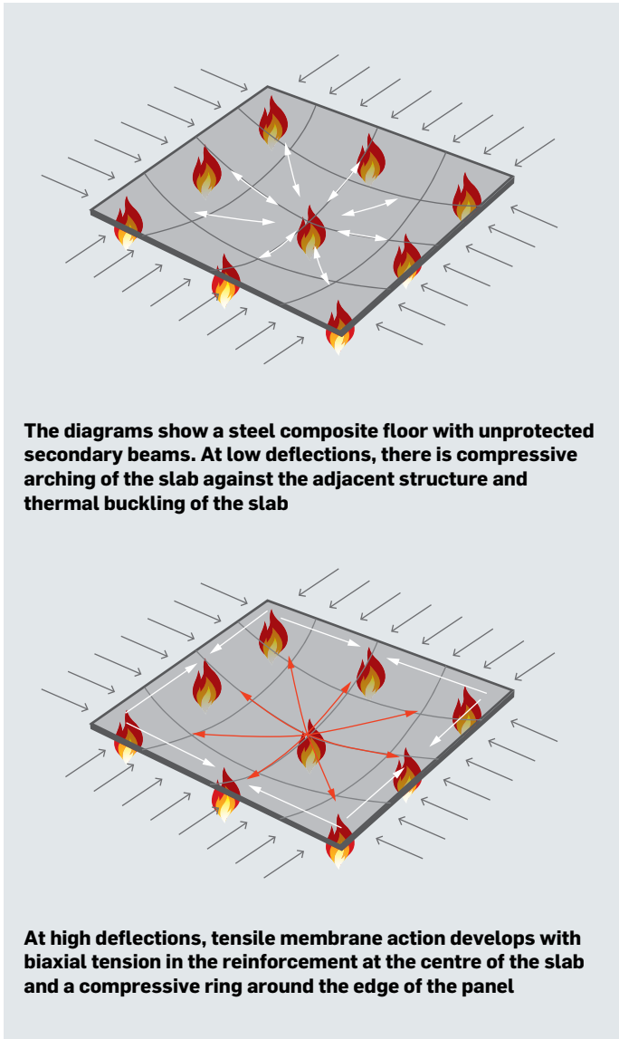
FIG 6. ENHANCED FIRE RESISTANCE IN STEEL COMPOSITE FLOORS
