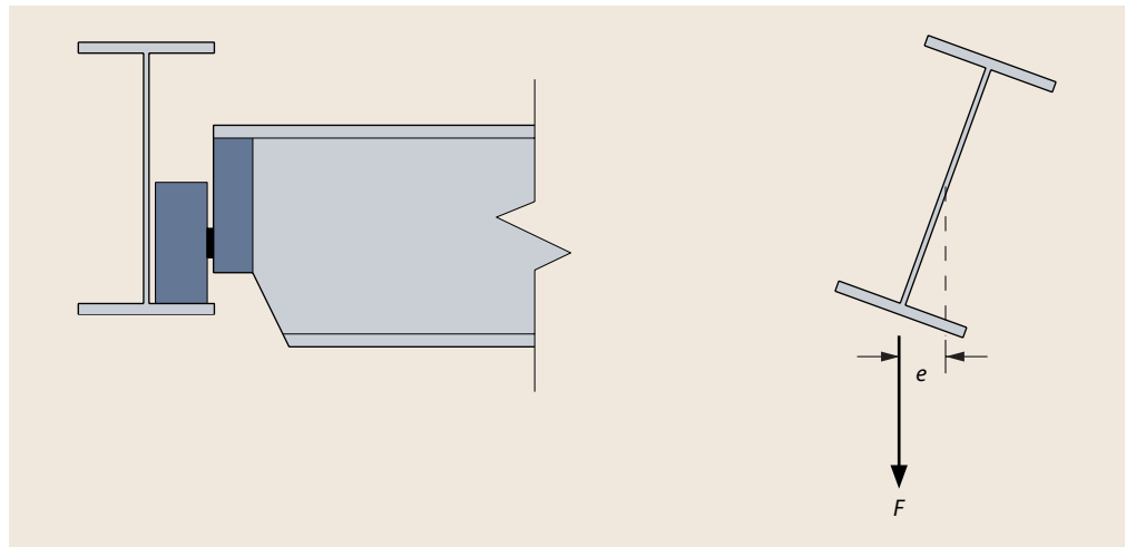
Figure 4.1 Stabilizing loads
