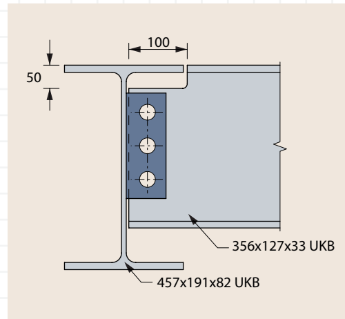
Figure 2.1 Connection details
