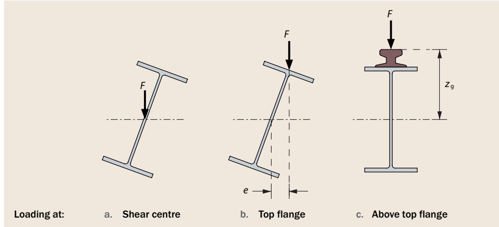
Figure 2.5 Effect of load level
