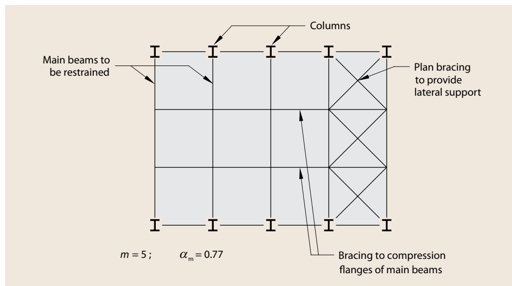
Figure 3.8 Plan bracing
