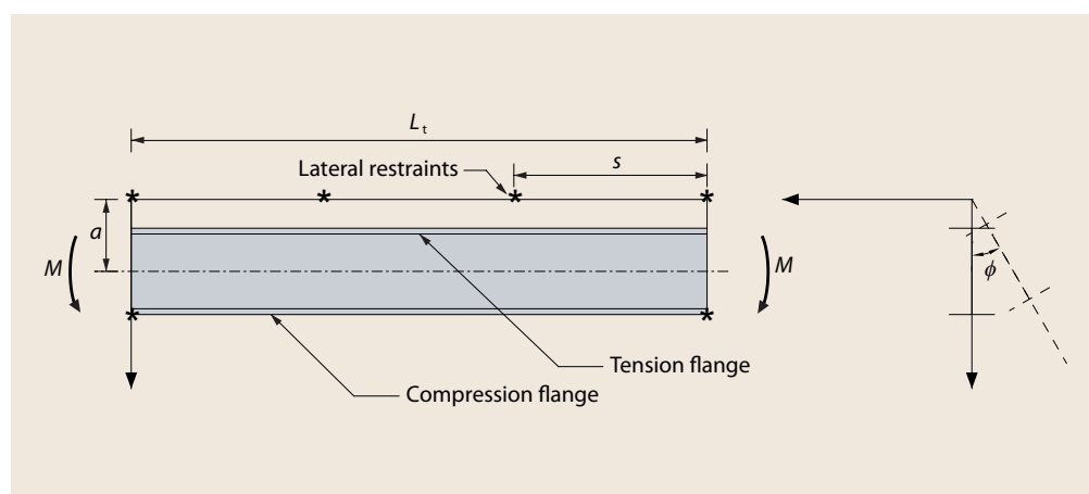
Figure 2.9 Buckling about a restrained axis adjacent to the tension flange
